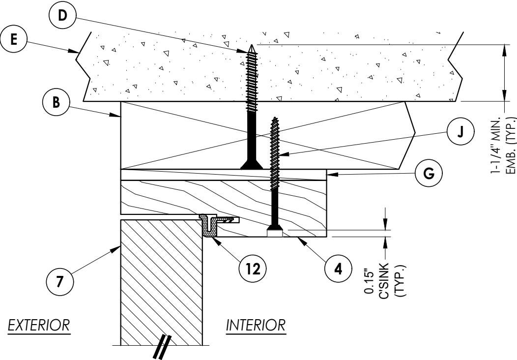
1 VERTICAL CROSS SECTION 4 Outswing shown
