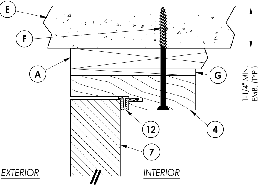
2 VERTICAL CROSS SECTION 4 Shown w/1X sub-buck
